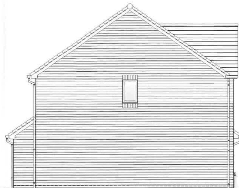
Left Elevation
